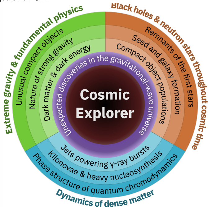
Figure 1. Graphical illustration of the science goals for CE.
