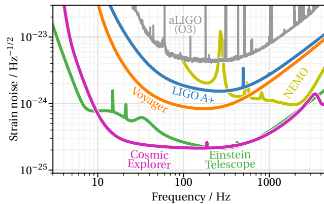
Figure 2. Strain sensitivity progression, LIGO to CE. [7]
