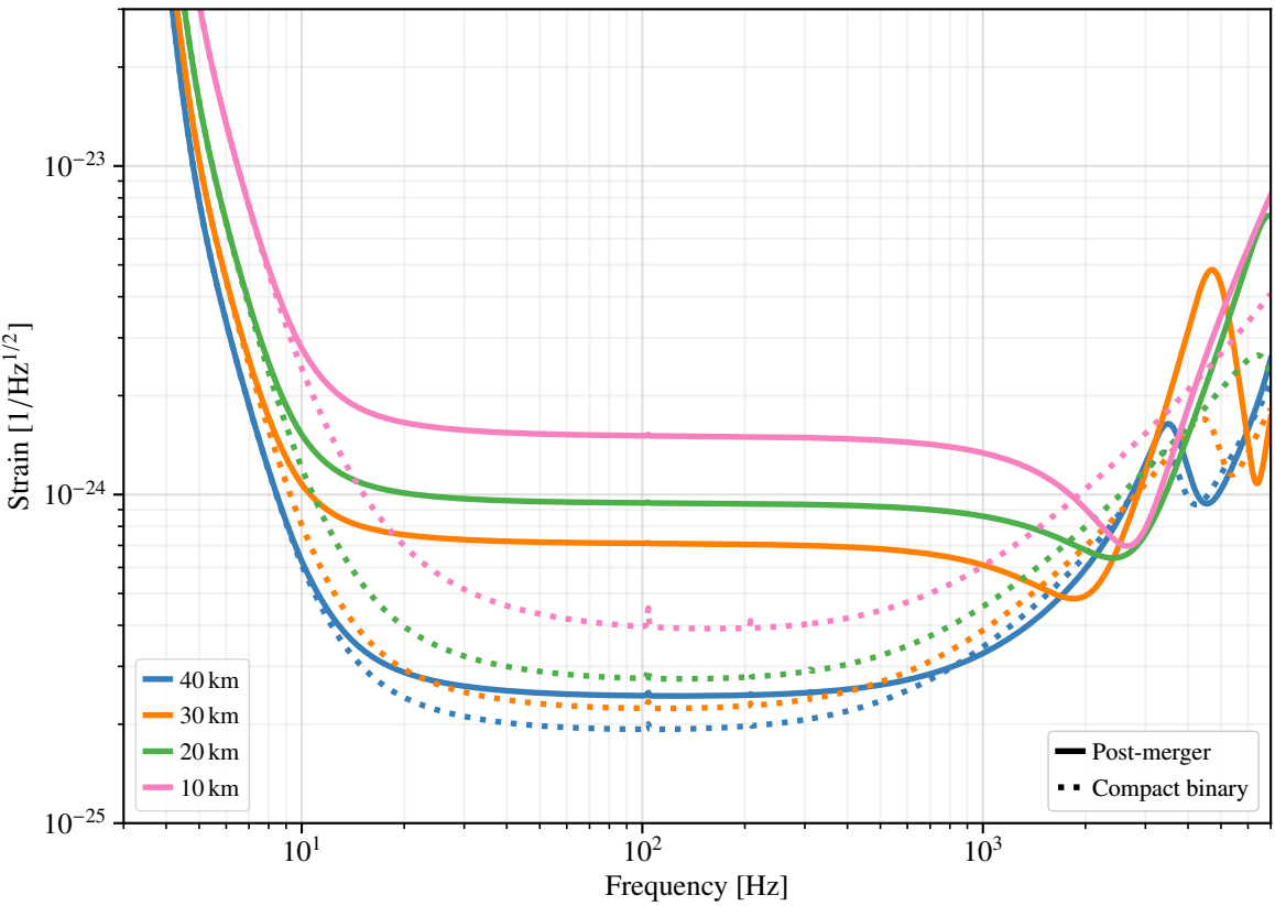
Cosmic Explorer 2 Sensitivity
