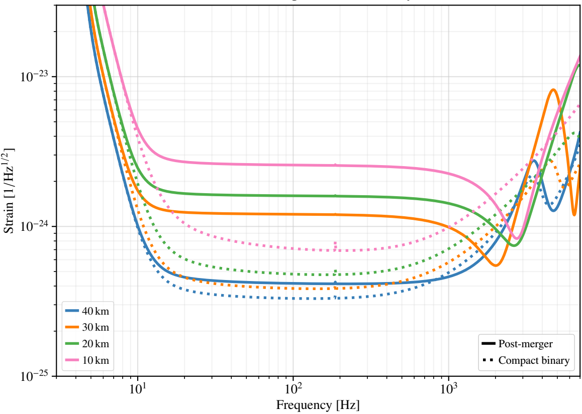
Cosmic Explorer 1 Sensitivity
